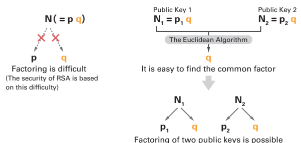
Figure 12: A System Allowing Third-Parties to Identify When Two Different Public Keys Share a Private Key.
