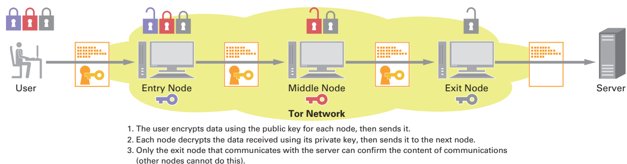
Figure 12: Encryption of Tor Communications
